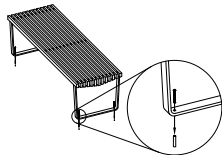
Floor Mount (FM01) - Concrete Application
