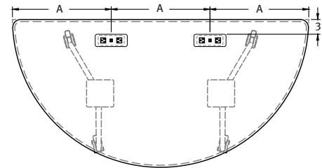
Half-Round Table - 2 Power Units
