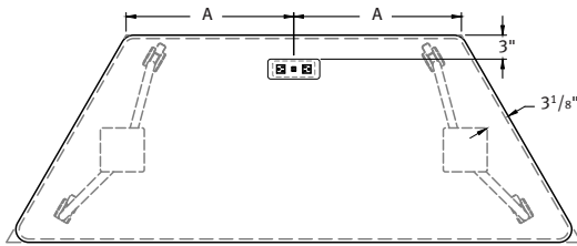
Trapezoid Table, Short Side - 1 Power Unit
