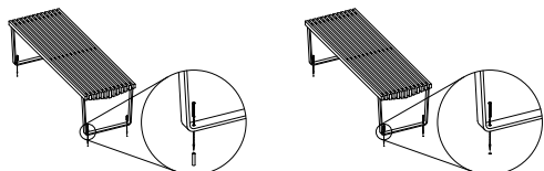
Floor Mount (-FM01) - Concrete Application Floor Mount (-FM02) - Wood Application
