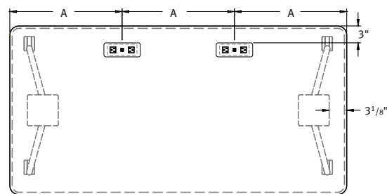
Rectangle Table - 2 Power Units
