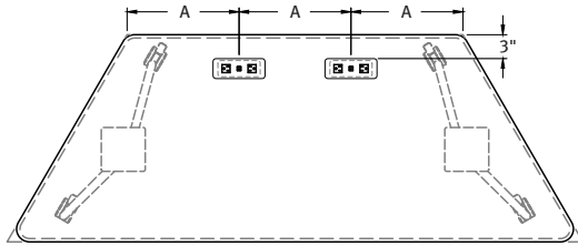
Trapezoid Table, Short Side - 2 Power Units
