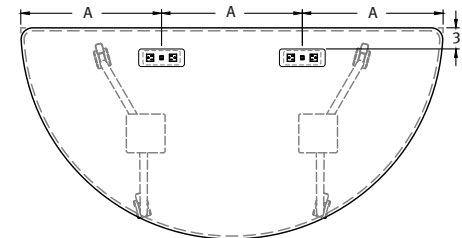
Half-Round Table - 2 Power Units
