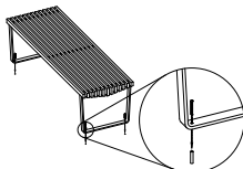
Floor Mount (-FM01) - Concrete Application
