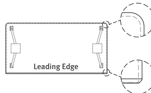
One-sided waterfall edge tables will have 90-degree corner on leading edge and radiused corner on opposing side
