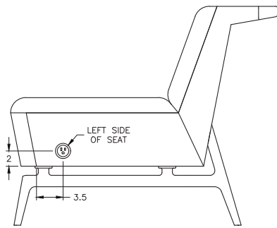
Side placement (armless models only)
