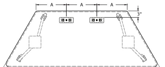
Trapezoid Table, Short Side - 2 Power Units
