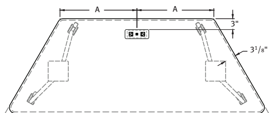
Trapezoid Table, Short Side - 1 Power Unit
